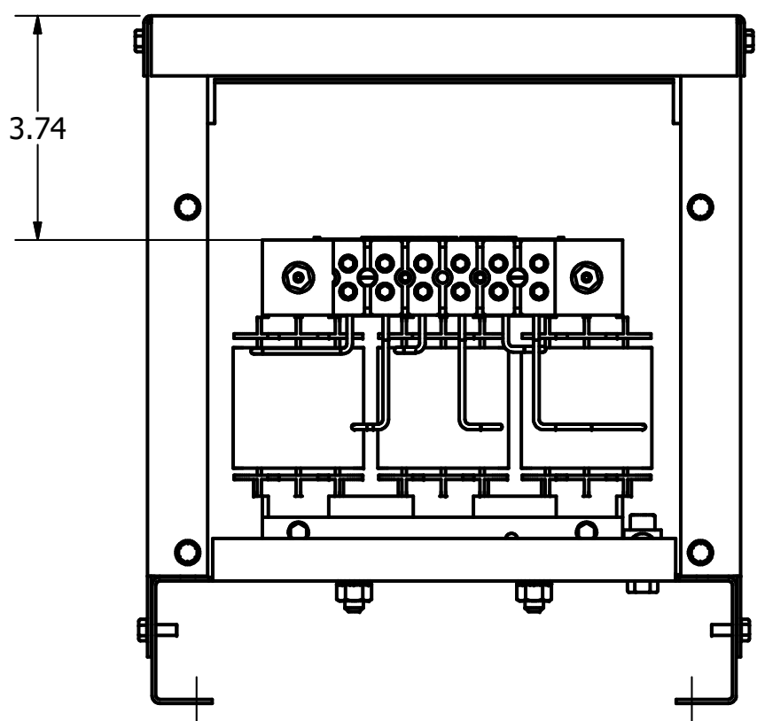
Front View Without Front Cover
