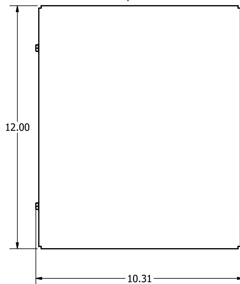
Top View
