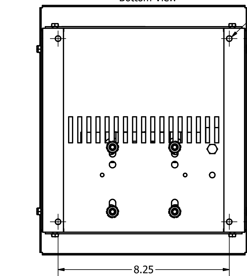
Bottom View
