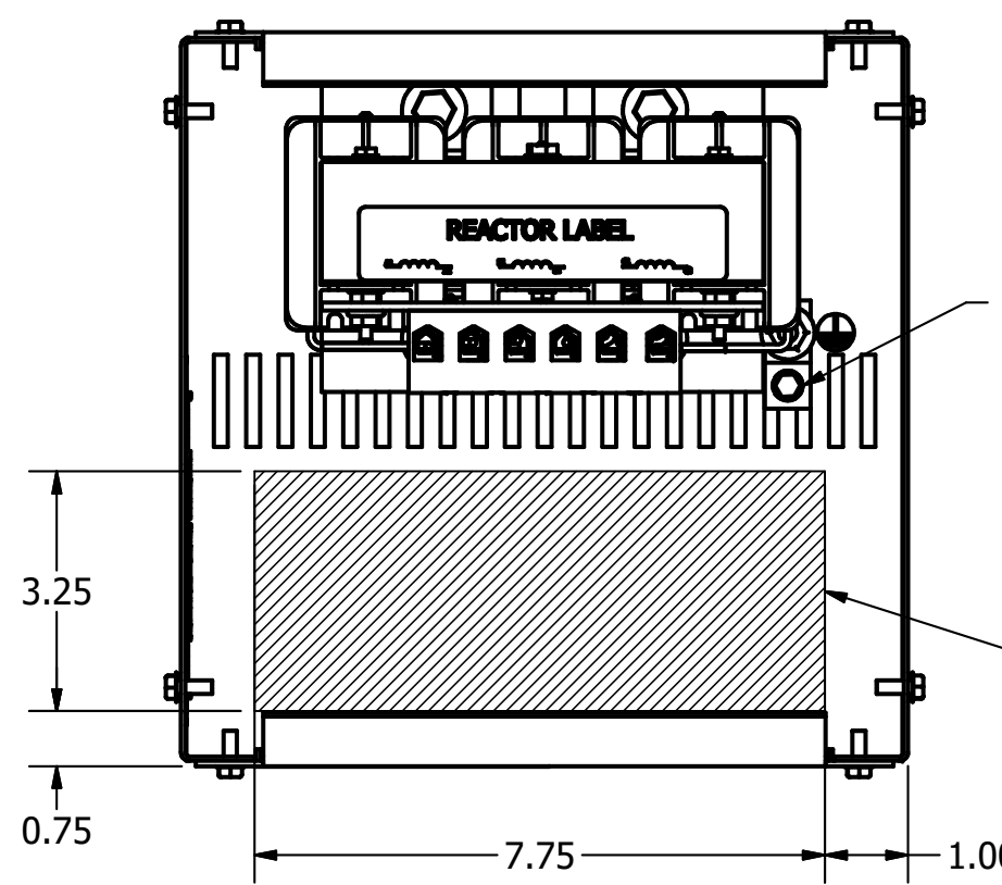
Front View Without Front Cover
